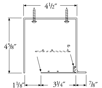
Cross Section of Type D Pocket
